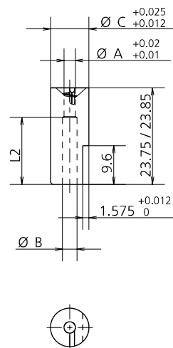
002 (8053) MATRICE / MATRIX / MATRIX HSS-62HRC
