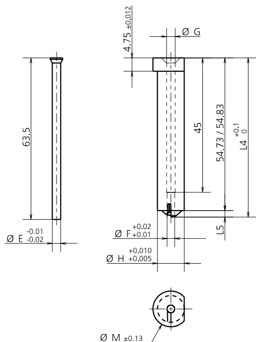
001 (8064) PUNZONE / PUNCH / LOCHER HSS-62HRC
