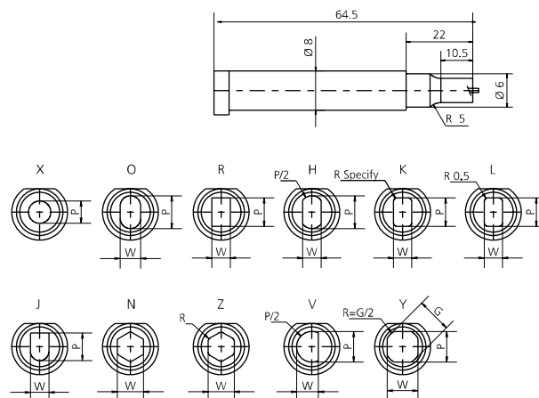
007 (09M) PUNZONE TC / HEADED PUNCH / SCHNEIDSTEMPEL ISO8020
